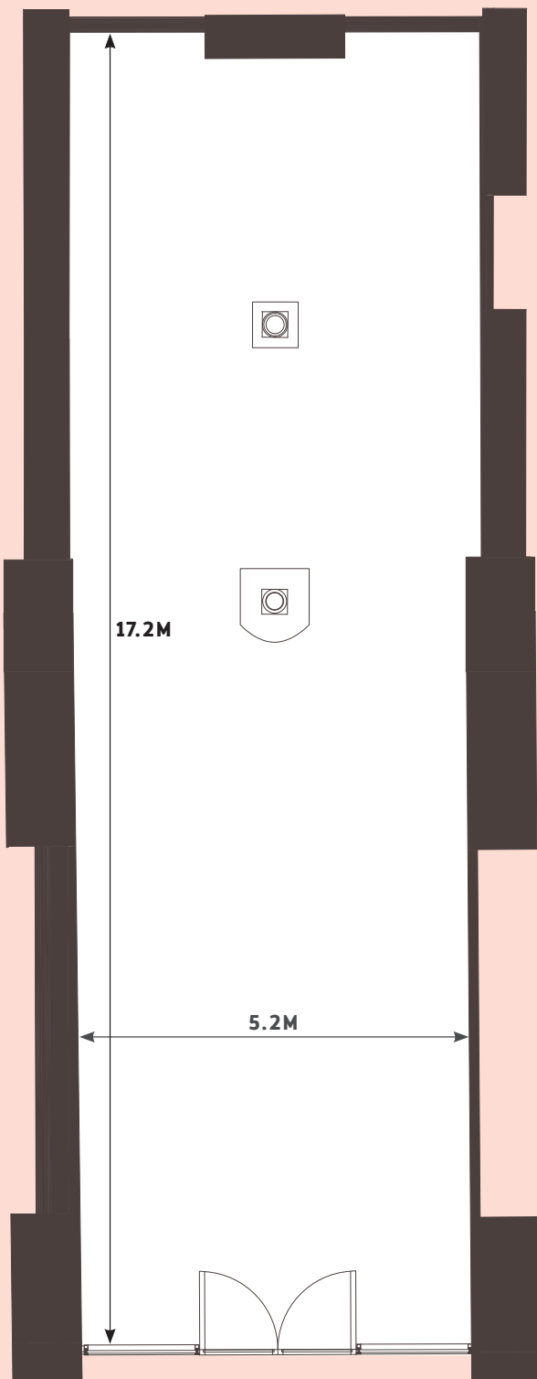
FLOOR PLAN
