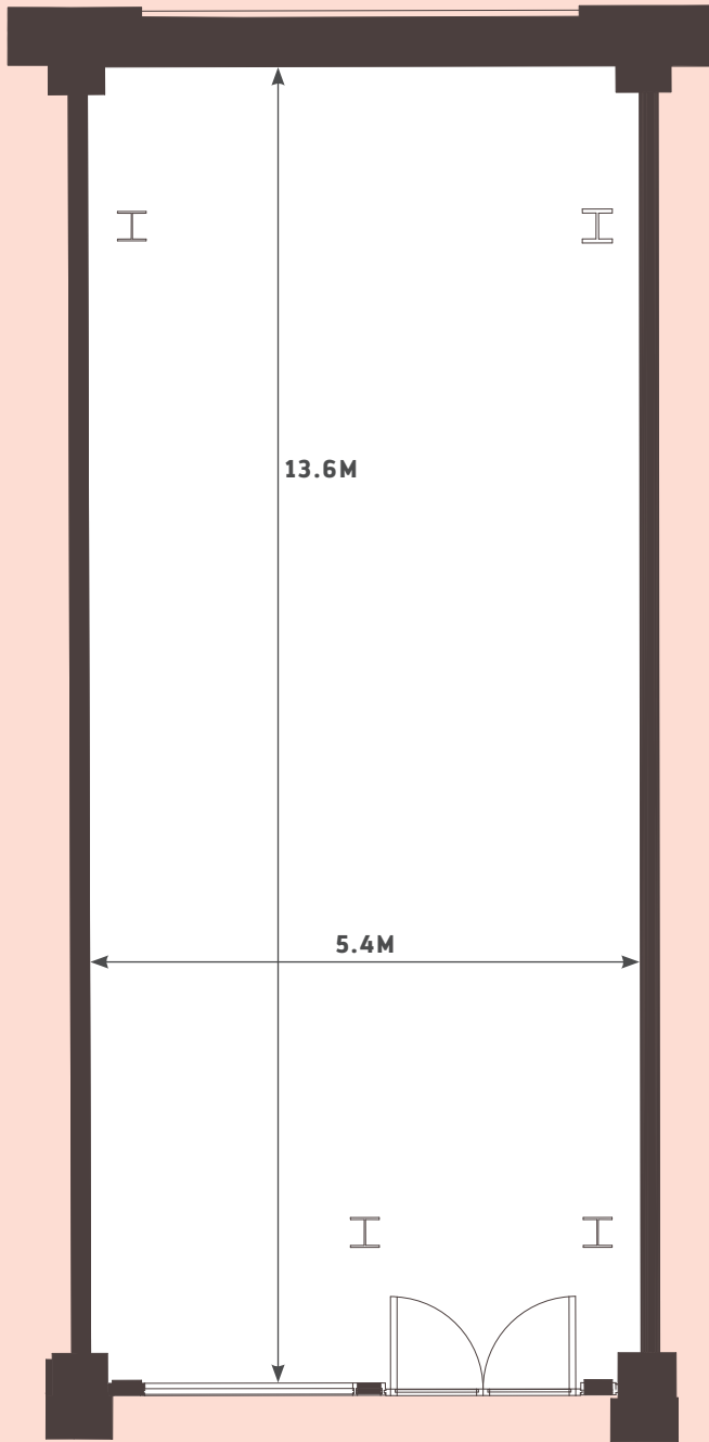
FLOOR PLAN
