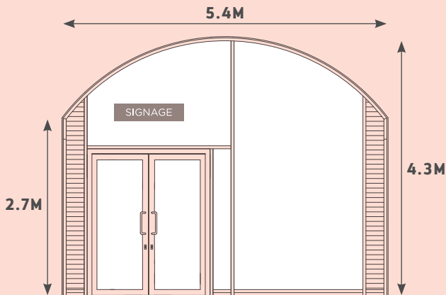
SHOP FRONT AND SIGNAGE ZONES
