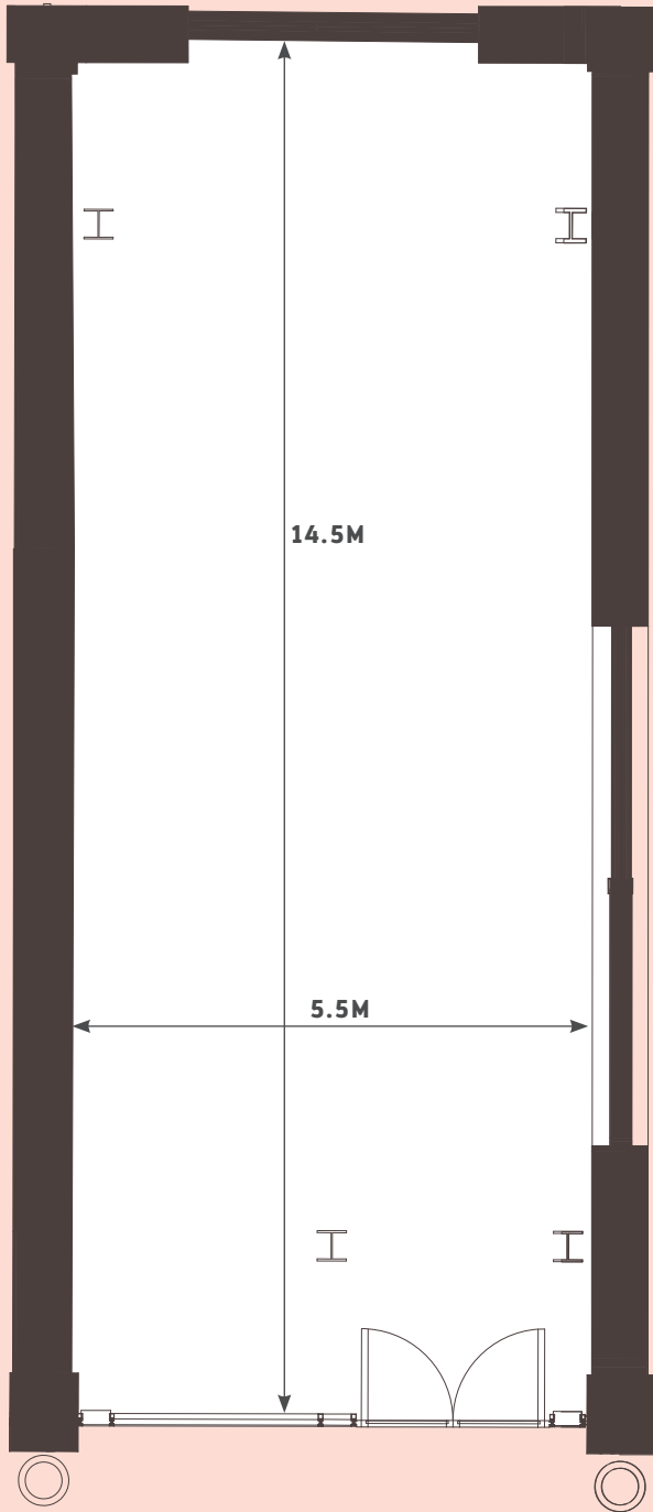
FLOOR PLAN
